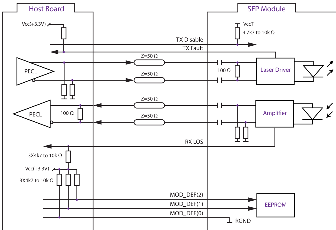
SFP Host Recommended Circuit
