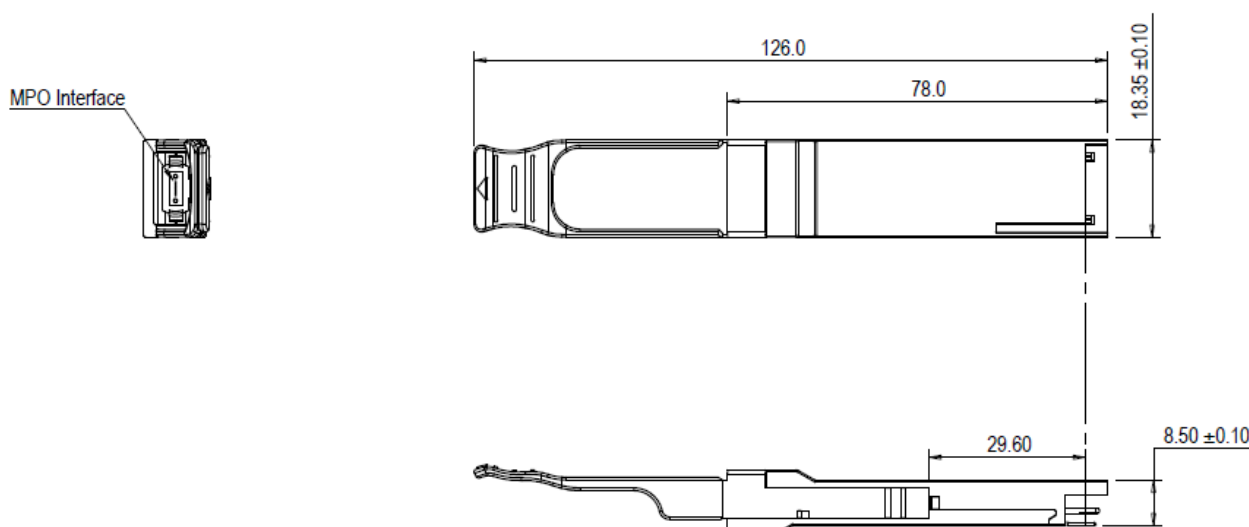
Figure 4. Mechanical Outline
