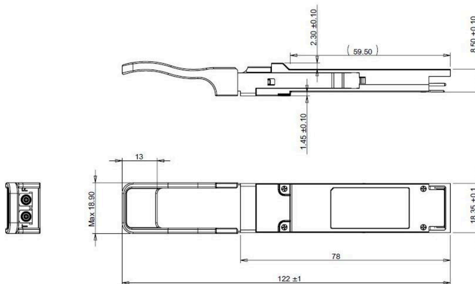
Figure 4. Mechanical Outline
