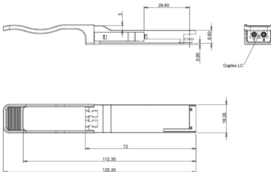
Figure 5. Mechanical Outline
