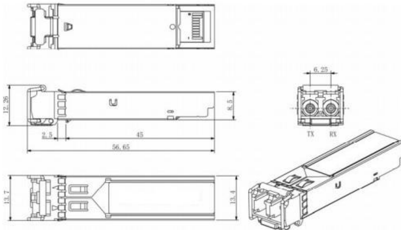
Figure 3. Mechanical Drawing
