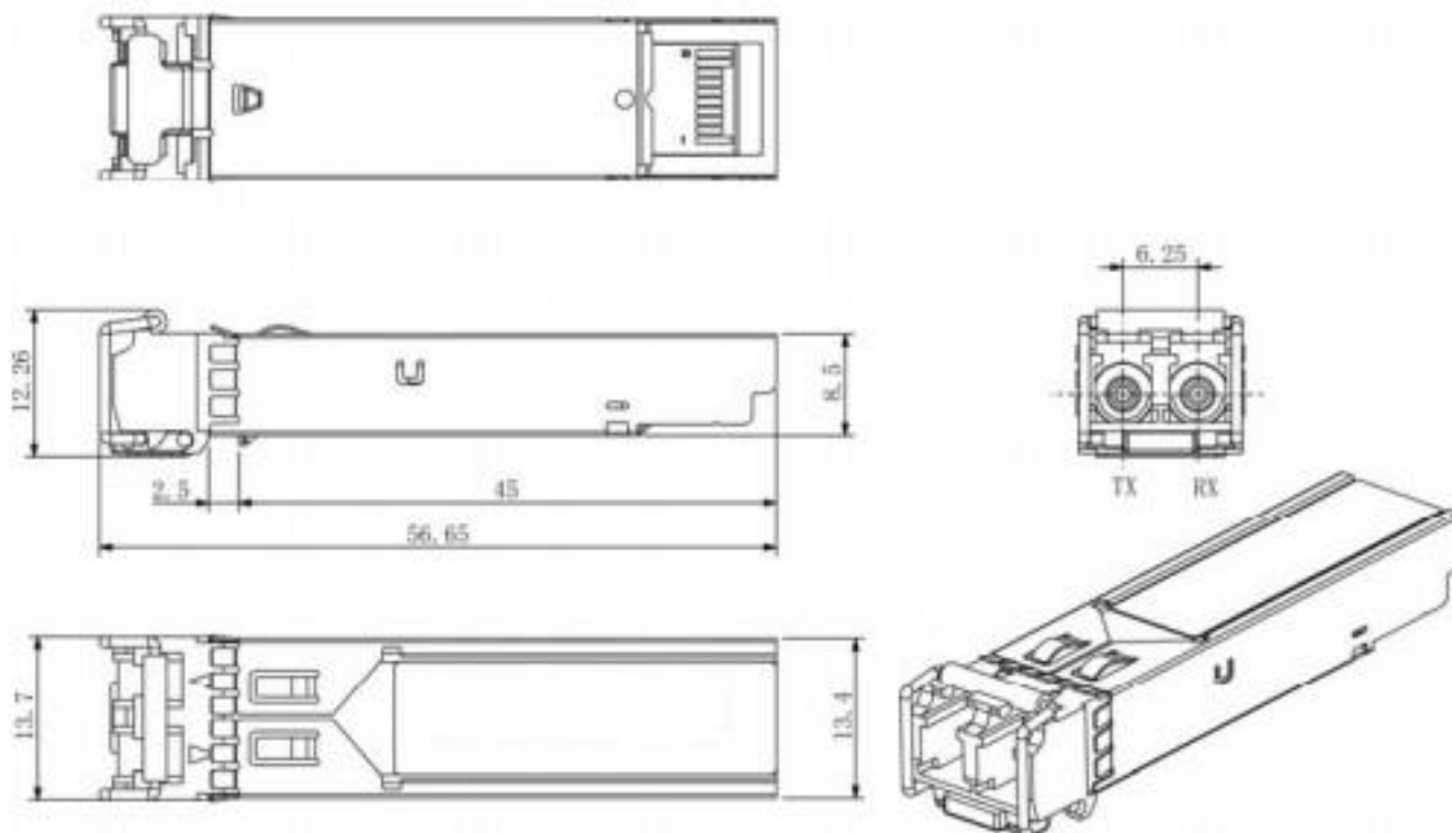
Figure 4. Mechanical Drawing
