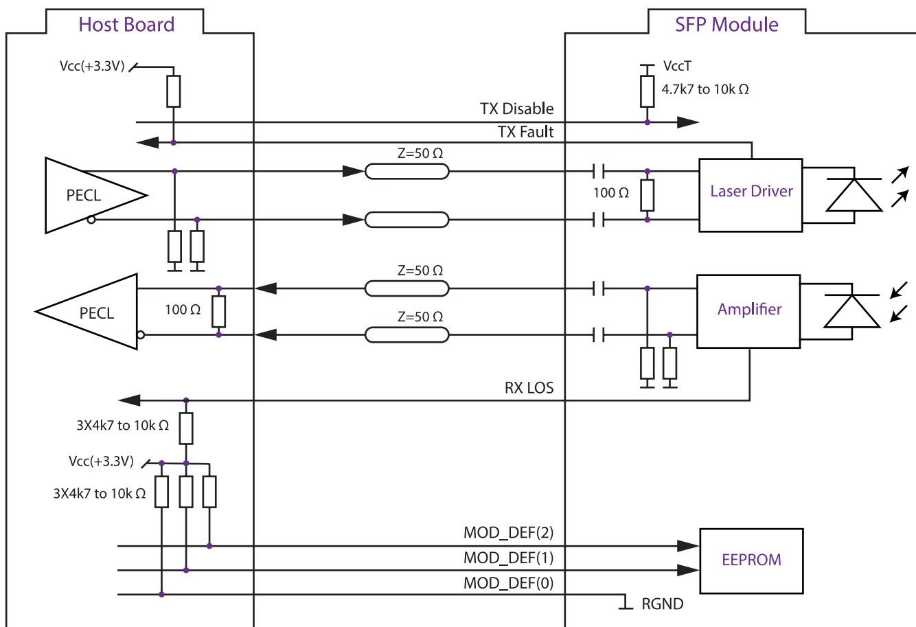
Figure 2. SFP Host Recommended Circuit
