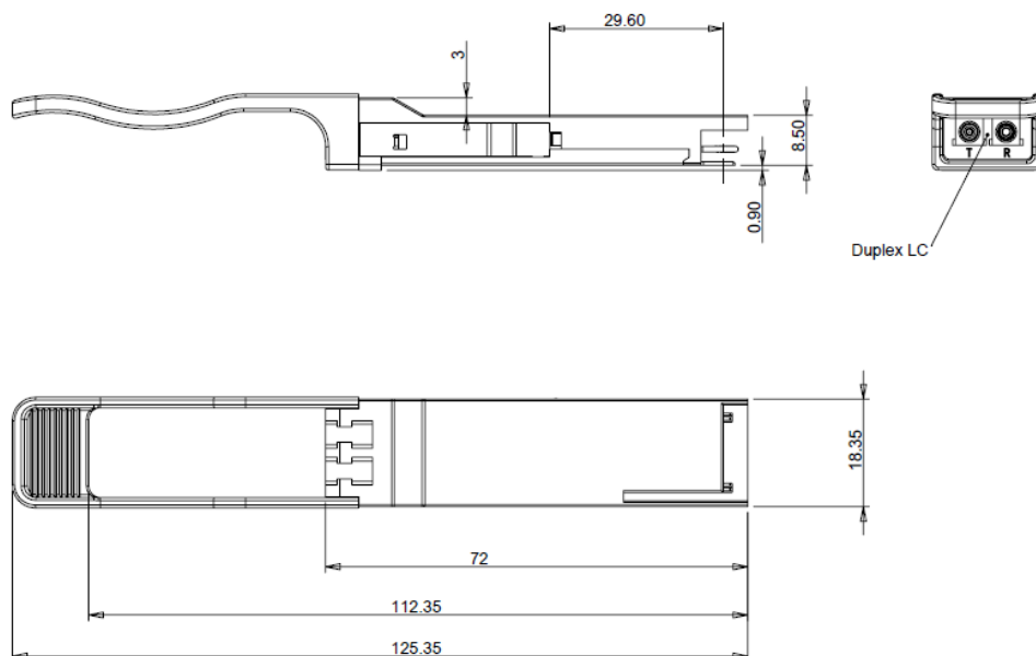
Figure 5. Mechanical Outline
