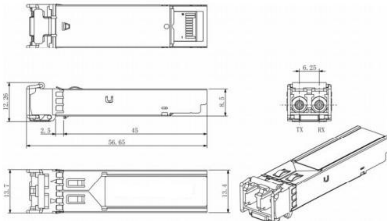
Figure 4. Mechanical Drawing
