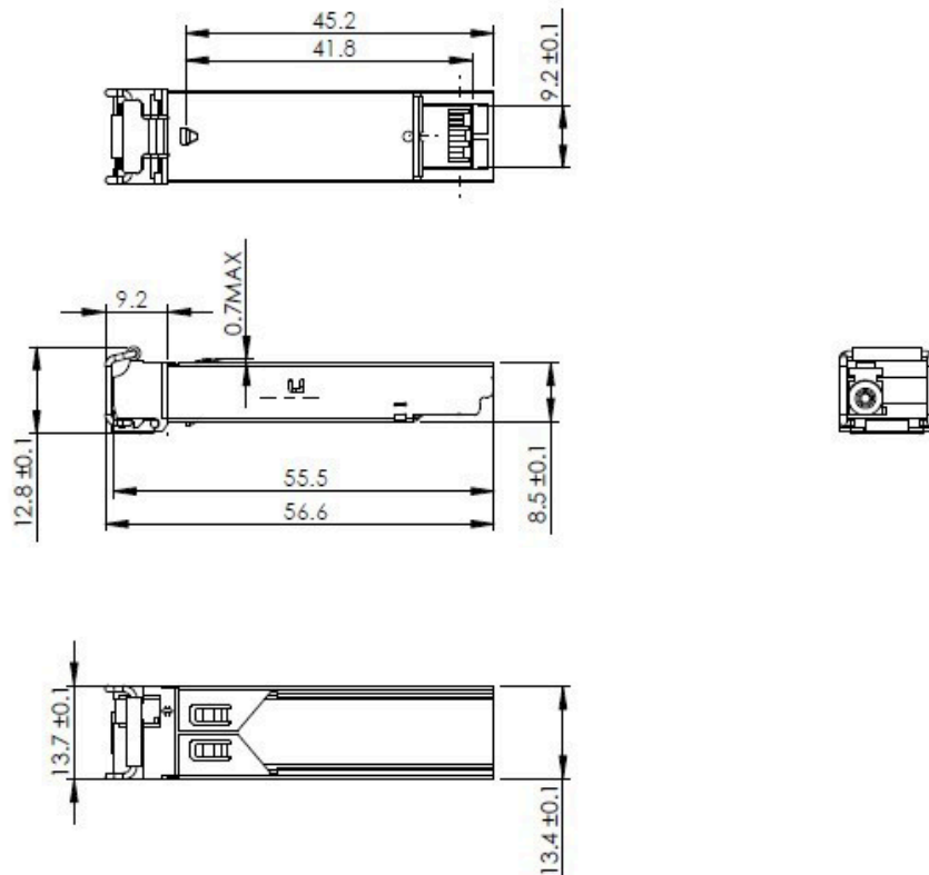
Figure 3. Mechanical Drawing
