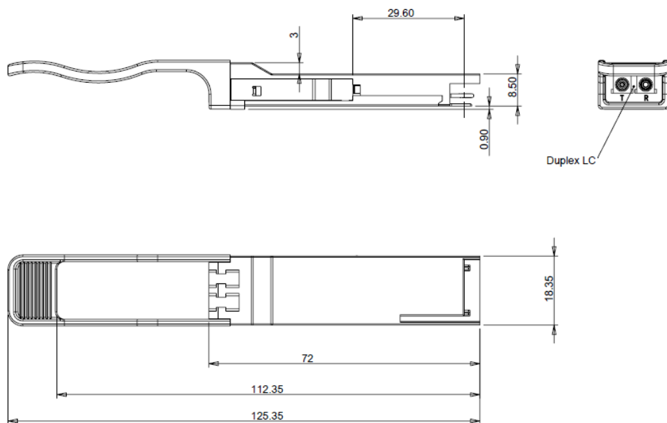
Figure 5. Mechanical Outline
