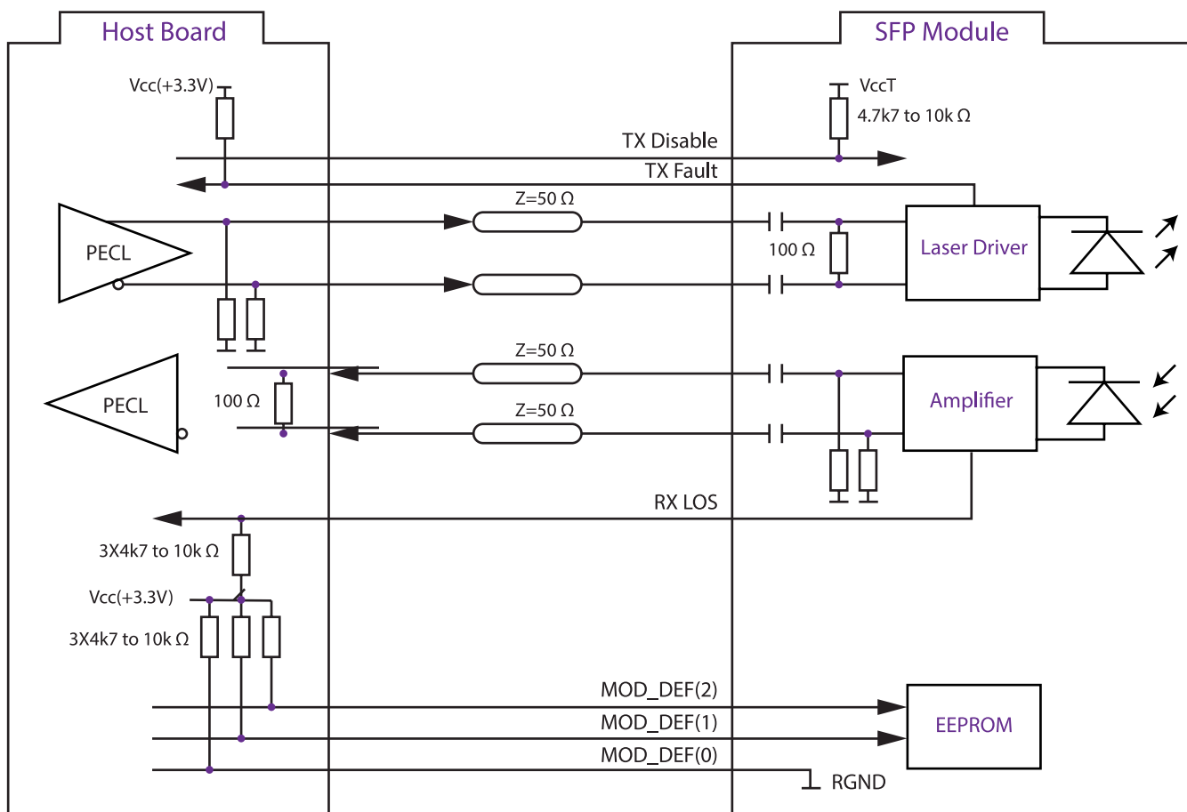
Figure 3. SFP Host Recommended Circuit
