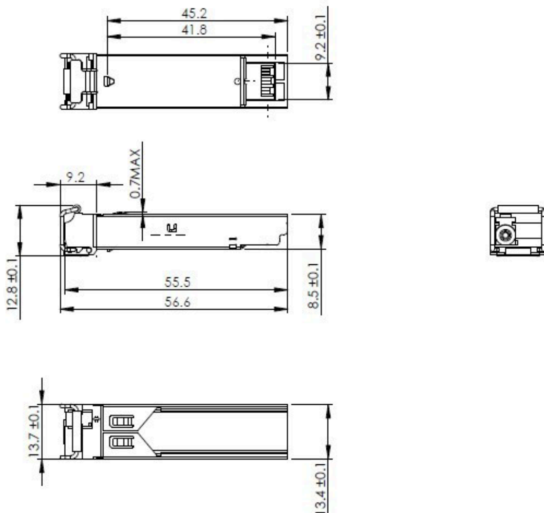
Figure 4. Mechanical Drawing
