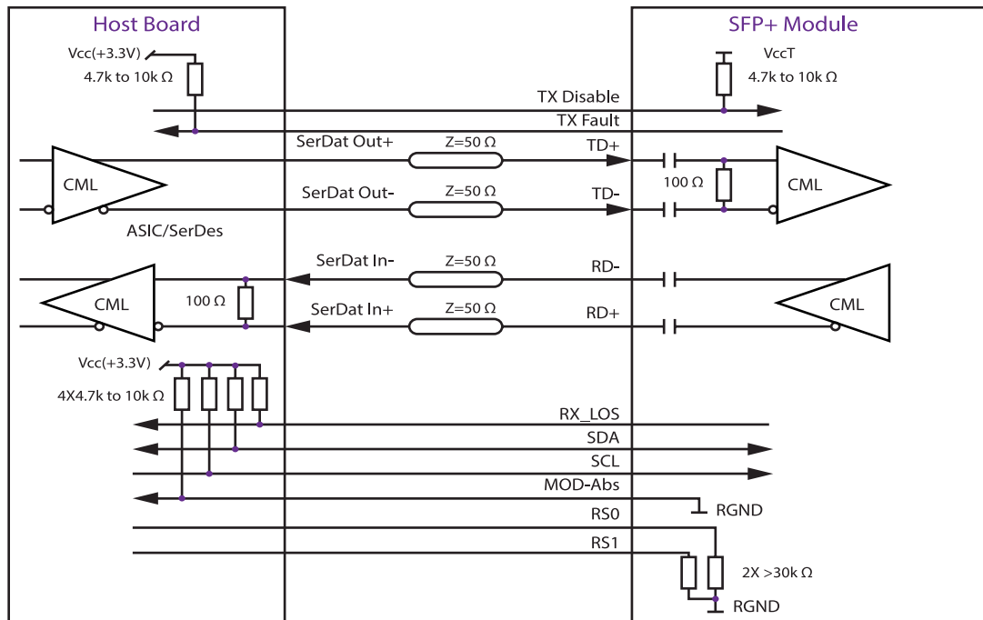
Figure 4: Recommended High-speed Interface Circuit
