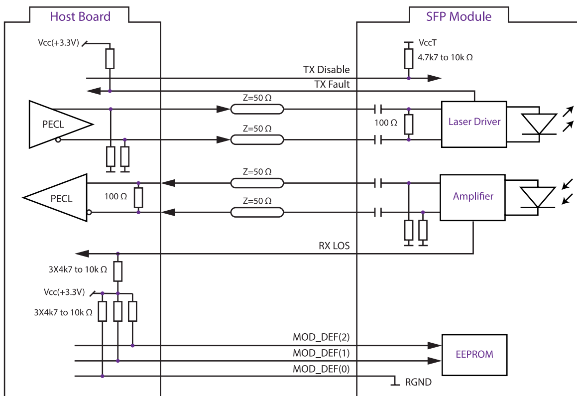
Figure 3. SFP Host Recommended Circuit
