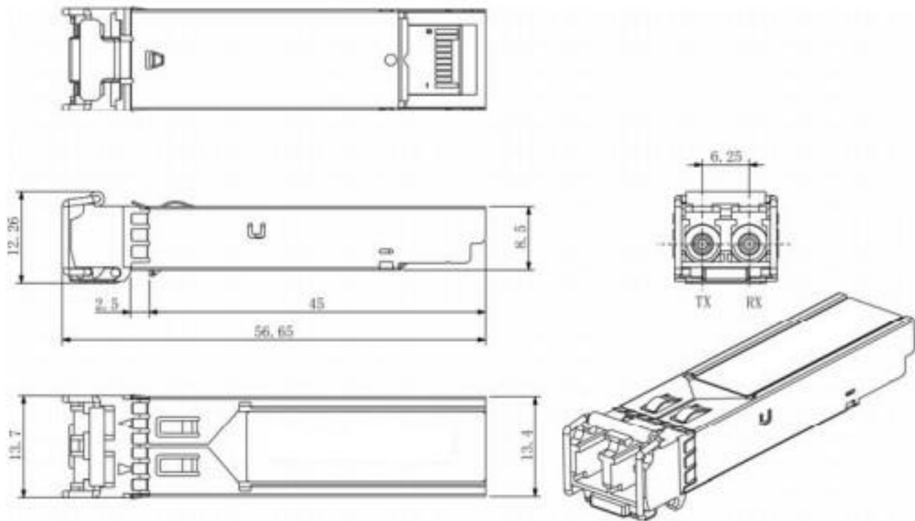
Figure 4. Mechanical Drawing
